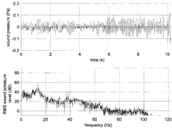
Figure 11. Event recorded at H1 shortly after Bag Plant 1 switched on.
