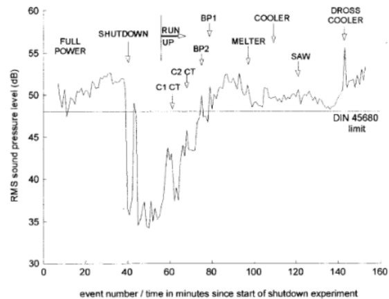
Figure 13. Variations in 40 Hz third-octave band level throughout shutdown experiment, with details of plant activity (C1 CT = Caster 1 Cooling Tower; C2 CT = Caster 2 Cooling Tower; BP1 = Bag Plant 1; BP2 = Bag Plant).
