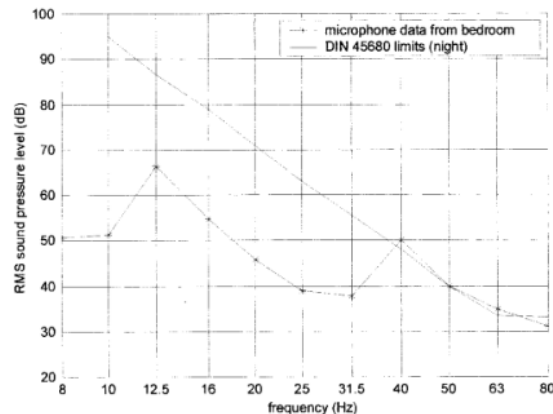
Figure 5. Typical third-octave band levels detected at house H1, compared with DIN 45680 limits.
