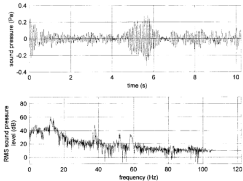
Figure 12. Event recorded at H1 shortly after Bag Plant 2 switched on.
