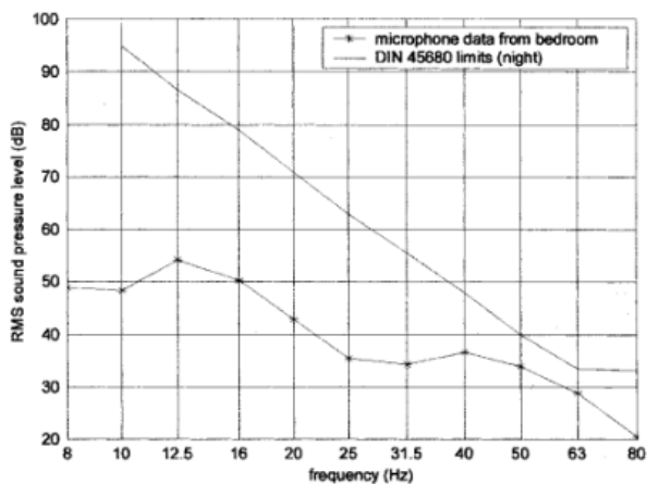
Figure 9 Event recorded at H1 immediately after shutdown, plotted as third-octave bands levels against DIN 45680 limits.
