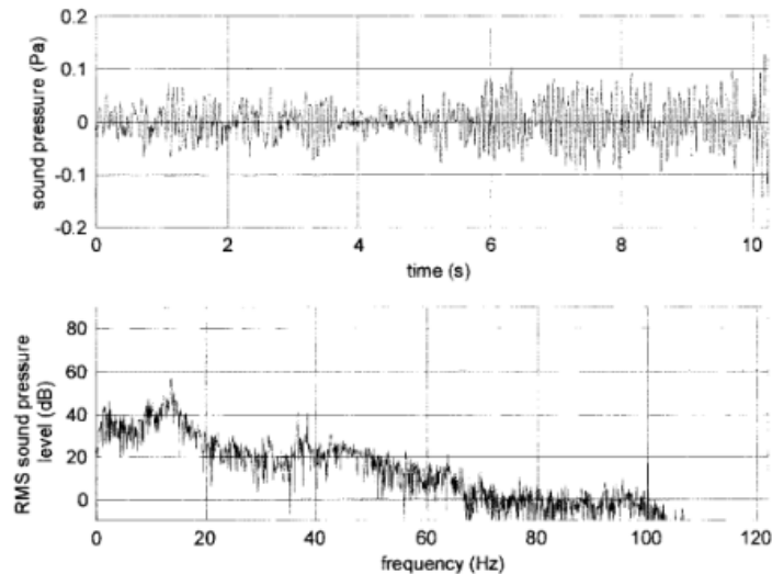
Figure 10 Event recorded at H1 shortly before Bag Plant switched on.
