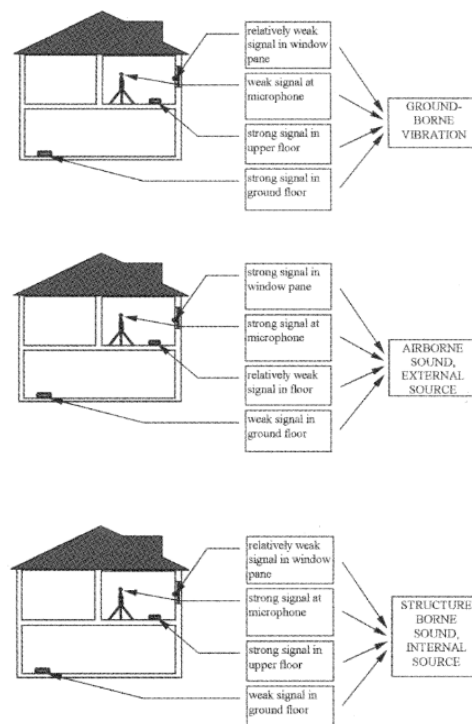
Figure 2. Identification of transmission paths and external/internal sources of low frequency noise/vibration 15
